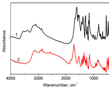
Figure 5. IR spectra of [\text{Nd}(\text{HTBA})_2(\text{C}_2\text{H}_3\text{O}_2)(\text{H}_2\text{O})_2] \cdot 2\text{H}_2\text{O} ( 1 ) and III polymorph modification of 2-thiobarbituric acid ( 2 ).
